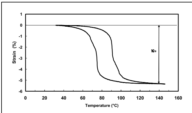
Figure 9 - Hysteresis measurement
