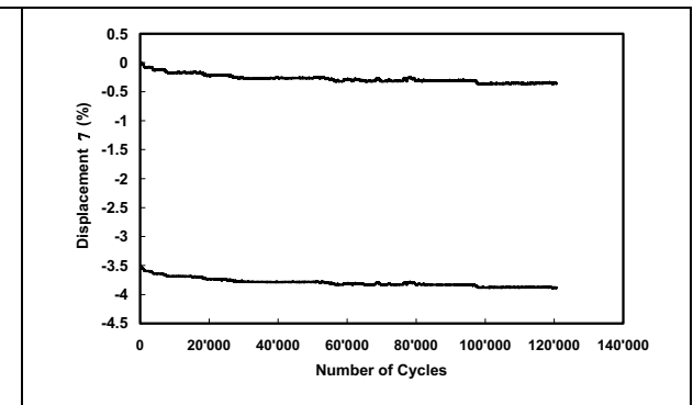
Figure 10 - Fatigue life test
